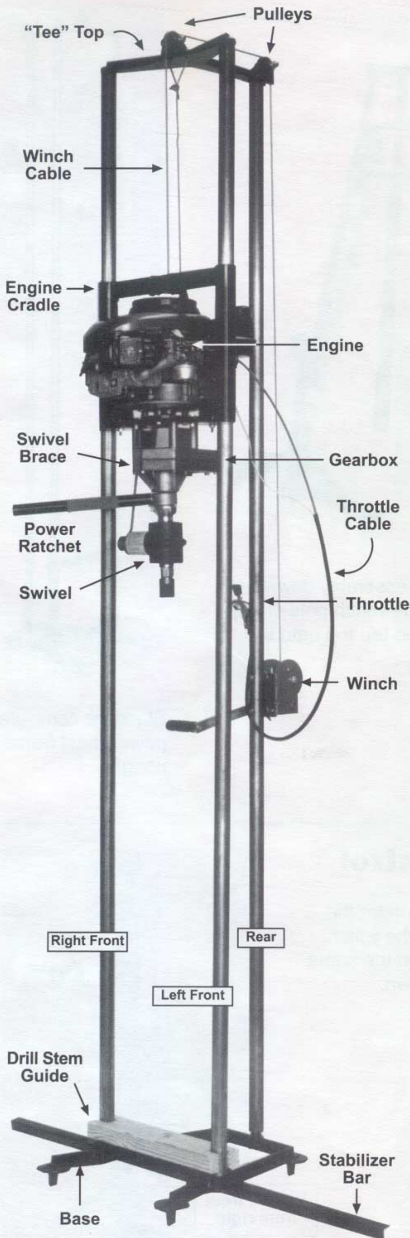
ASSEMBLED POWER MAST (Front View)
